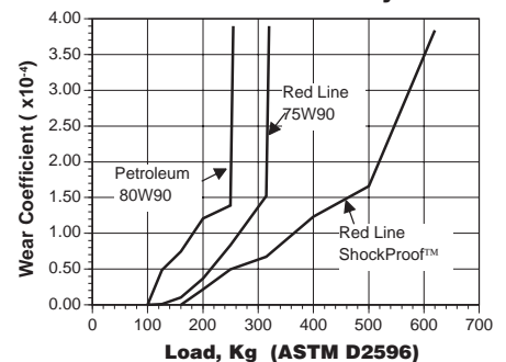
Coefficient of Wear - Heavy Loads
